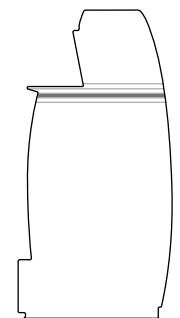
LEVEL 53 SOUTH ELEVATION
